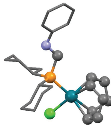
Fig. 4 X-Ray structure of (\text{C}_6\text{H}_{11})_2\text{PCH}_2\text{NHPPhRh}(\text{cod})\text{Cl} [CCDC 748467]. 51
