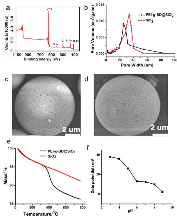
Fig. 1 The synthesized materials were characterized by X-ray photoelectron spectroscopy (a), scanning electron microscopy (silica before (c) and after modification (d), thermogravimetry analysis (e) and zeta potential analysis (f).
