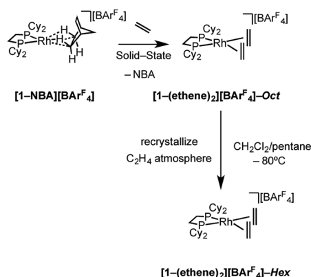
Scheme 4 Synthesis of [1-(\text{ethene})_2][BARF_4] as octahedral ("Oct", C_2/c ) and hexagonal ("Hex", P6_322 ) polymorphs.
