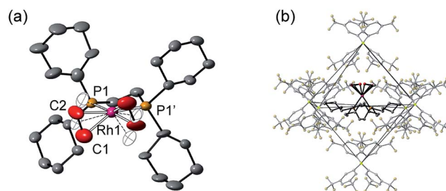
Fig. 1 Solid-state structure of [1-(\text{ethene})_2][BARF_4]\text{-Oct} . (a) Cation showing the numbering scheme, displacement ellipsoids shown at the 50% probability level, 50% disorder component shown as open ellipsoids. (b) Local environment around the cation showing the arrangement of [BARF_4]^- anions. H-Atoms are omitted.
