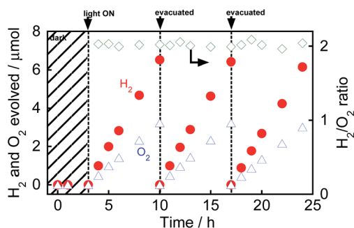
Fig. 1 Time courses of evolution of \text{H}_2 and \text{O}_2 from water over \text{Au(1.0)/TiO}_2 under irradiation with visible light from a Xe lamp with an L-42 filter. After 10 h and 17 h of irradiation and evacuation, the suspension was irradiated again.
