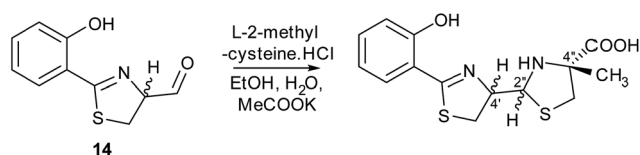
Scheme 1 Synthesis of an authentic standard of (4'' R )-isopyochelin as a mixture of stereoisomers at C-4' and C-2''.
