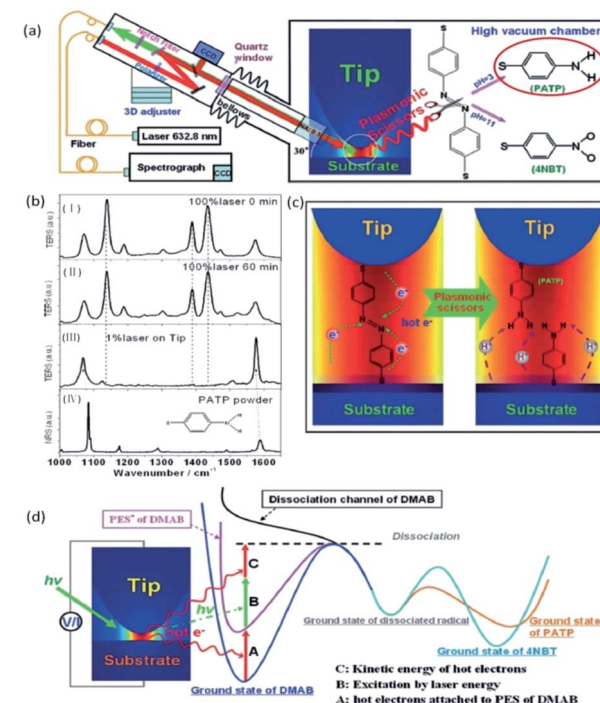
Fig. 10 (a) Schematic of DMAB separated by HV-TERS as plasmonic scissors. (b) TERS and NR spectra under different conditions. TERS spectra of DMAB at 0 min (I) and 60 min (II), TERS of PATP on the tip with 1% power excitation for 60 min (III) NRS of PATP powder (IV). (c) Dynamic process of DMAB dissociating to PATP by HV-TERS. (d) Schematic of the process paths of DMAB dissociated to PATP. 58
