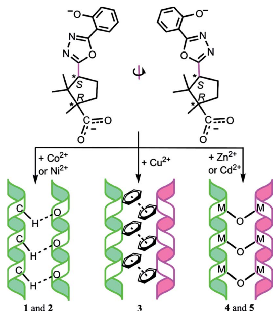
Scheme 15 Conformational twists of the asymmetric skeleton of (1 R ,3 S )-1,2,2-trimethyl-3-[(5-(2-hydroxy) phenyl-1,3,4-oxadiazol-2-yl)]cyclopentanecarboxylic acid and different interhelical interactions in the prepared CPs. [Reprinted with permission from ref. 202. Copyright 2012, American Chemical Society.]
