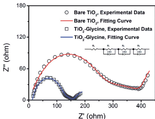
Fig. 28 Nyquist plots of perovskite solar cells based on bare \text{TiO}_2 (symbol B) and glycine-treated \text{TiO}_2 (symbol). Symbols are experimental data and solid lines correspond to the fitting results using the equivalent circuit shown in the inset figure. EIS spectra were recorded using a potentiostat/galvanostat instrument (PGSTAT 302N, Autolab) equipped with a FRA2 module under constant light illumination of 100 \text{ mW cm}^{-2} . A DC applied bias voltage was set at open circuit voltage of the perovskite solar cells with a sinusoidal ac potential perturbation of 15 mV over a frequency range from 1 MHz to 0.01 Hz. 137
