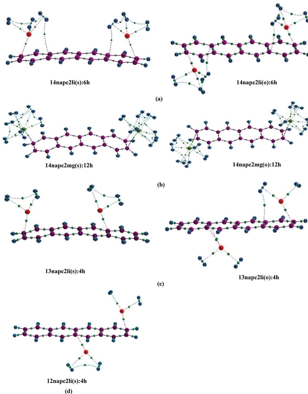
Fig. 7 Electron density molecular graphs of (a) Li^+ -decorated on 'R1–R4', (b) Mg^{2+} -decorated on 'R1–R4', (c) Li^+ -decorated on 'R1–R3', (d) Li^+ -decorated on 'R1–R2' position of naphthalene with maximum number of H_2 molecules at CAM-B3LYP level in conjunction with 6-311+G(d,p) basis set. The green dot localized between the H_2 and the metal ion indicates the location of bond critical point of the electron density.
