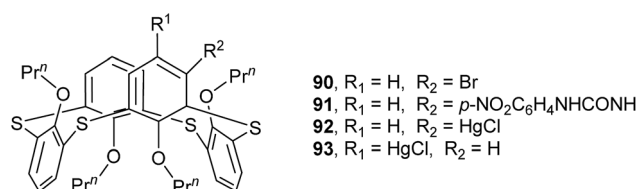
Fig. 80 Structures of compounds 90 – 93 .
