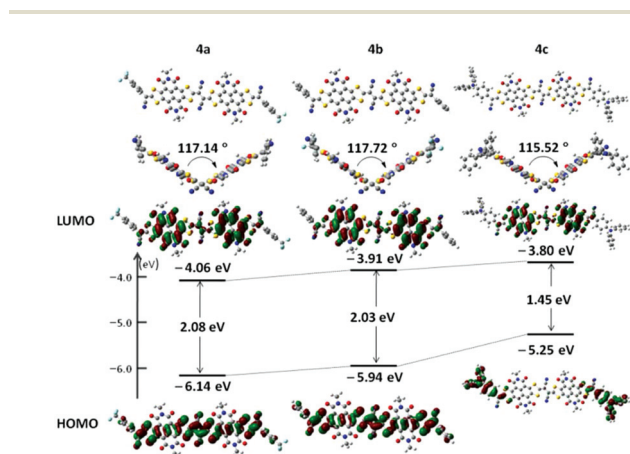
Fig. 2 Molecular geometries, frontier molecular orbitals and the energy level diagram of N,N' -bis(methyl)-substituted model molecules for 4a–c , obtained by DFT calculations.
