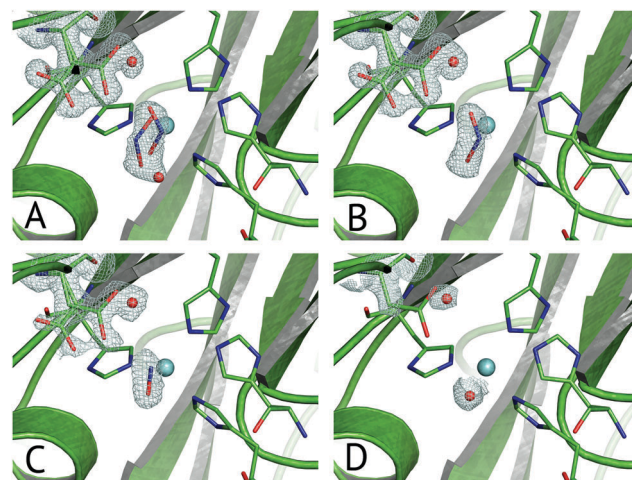
Fig. 7 Selected frames from the 45-frame MSOX structural movie of AcNiR catalysis at 100 K. 55 (A) The starting nitrite-bound state with partial occupancies in the top-hat and side-on modes (dataset 1, PDB 5i6k); (B) fully side-on nitrite (dataset 4, PDB 5i6l); (C) side-on nitric oxide product complex (dataset 17, PDB 5i6n); (D) water rebinding to the T2Cu following dissociation of NO (dataset 40, PDB 5i6k). Electron density is shown, contoured at 0.53–0.36 e − Å −3 , for the ligands and the Asp CAT residue, present in its ‘gatekeeper’ and ‘proximal’ orientations. The T2Cu atom is depicted by the cyan sphere and water molecules by red spheres.
