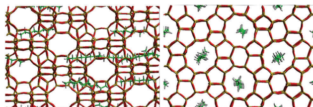
Fig. 3 A view of the system for octane in silicalite-1 pre-production run at 300 K viewed down the (left) 010 direction and (right) 100 direction. Reproduced from ref. 51 with permission from the PCCP Owner Societies.
