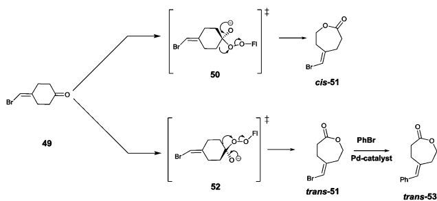
Scheme 17 Site-selective \sigma -bond migration in the Baeyer–Villiger reaction of ketone 49 leading to cis - and trans -configured olefins 51 and 53 via transition states 50 and 52 , respectively. 70
