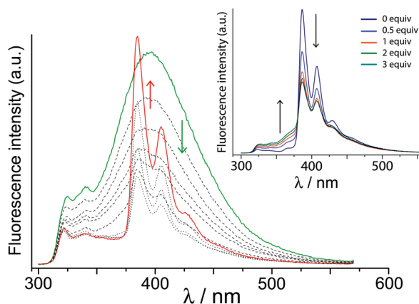
Fig. 3 Main figure: changes in fluorescence during addition of 3 to a solution of cage H (1 \mu M) in water resulting in formation of H : 3 : the cage fluorescence (green) is progressively quenched, and sensitised fluorescence from 3 (red) grows in. Inset: Restoration of fluorescence of cage H , and loss of sensitised pyrene fluorescence, on addition of cycloundecanone (3 equiv.) which displaces guest 3 from the cavity of H .
