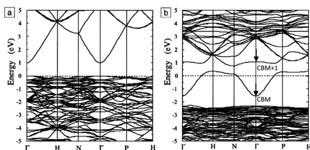
Fig. 2 Band structures of (a) undoped and (b) Sn-doped \text{In}_2\text{O}_3 . The Fermi level is set at E = 0 eV. The Brillouin zone centre is denoted by \Gamma , while H , N and P denote points at the Brillouin surface along high symmetry k -vectors in the reciprocal crystal lattice. The energy lines represent allowed electronic states at given k -points. Adapted with permission from Freeman et al. 6 Copyright 2011 Cambridge University Press.
