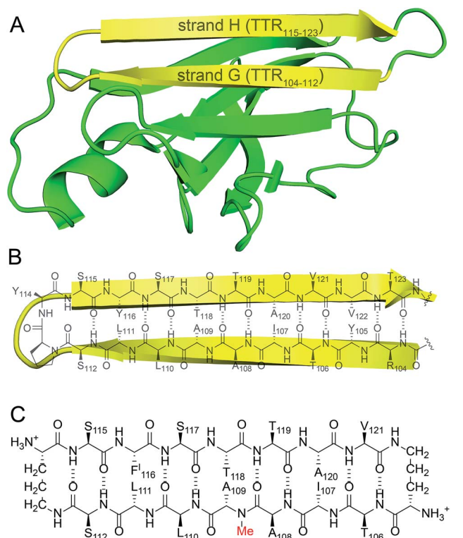
Fig. 2 (A) TTR monomer. The \beta -hairpin comprising \beta -strands G and H is highlighted in yellow. (B) Cartoon and chemical structure of the \beta -hairpin comprising \beta -strands G and H. (C) Chemical structure of peptide 1 .
