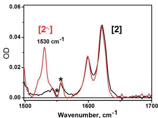
Fig. 3 IR spectra of 2 (black line) and electrochemically generated 2 1- (red line) recorded in CH 2 Cl 2 solutions containing 0.2 M [ 17 Bu 4 N][BF 4 ] electrolyte. The asterisks refer to incomplete solvent subtraction.
