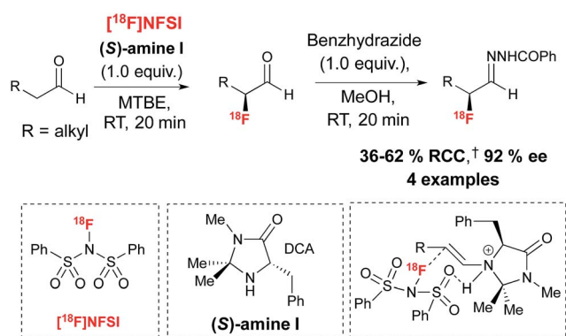
Scheme 5 Chiral imidazolidinone ( S )-I for the enantioselective ^{18}\text{F} -fluorination of aldehydes with ^{18}\text{F} -NFSI. ^{\dagger} RCC determined by radio-HPLC relative to ^{18}\text{F} -NFSI. DCA = dichloroacetic acid. For ^{18}\text{F} -NFSI, SA = 0.05 Ci \mu\text{mol}^{-1} , ( n = 3 ).
