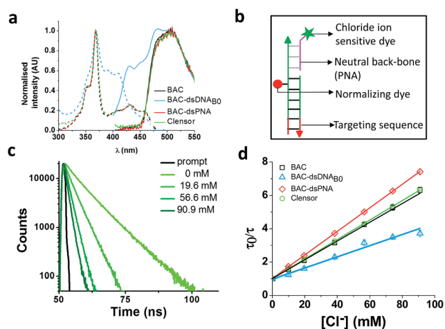
Fig. 4 (a) Comparison of excitation and emission spectra of BAC, \text{BAC-dsDNA}_{\text{B0}} , \text{BAC-dsPNA} and Clensor . (b) Schematic of Clensor . (c) Representative fluorescence lifetime decay traces of 1 \mu\text{M} Clensor in 10 mM potassium phosphate buffer, pH 7.2 at various chloride concentrations ( \lambda_{\text{ex}} = 443 \text{ nm} , \lambda_{\text{em}} = 488 \text{ nm} ). (d) Stern–Volmer plots for BAC, \text{BAC-dsDNA}_{\text{B0}} , \text{BAC-dsPNA} and Clensor . Average lifetime has been used to evaluate K_{\text{SV}} and k_{\text{q}} . Error bars indicate the mean of three independent experiments \pm s.e.m.
