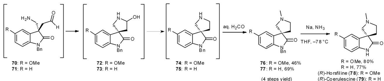
Total yield: (R)-Horsifiline 33%, (R)-Coerulescine 46% over three one-pot sequences
