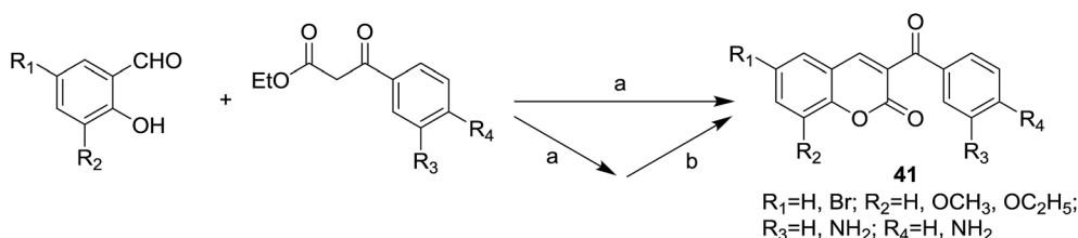
Scheme 2 Synthesis of antibacterial coumarin-chalcone hybrids. (a) EtOH, piperidine, reflux, 2–5 h; (b) SnCl_2 \cdot 2H_2O , EtOH, reflux, 3–7 h.
