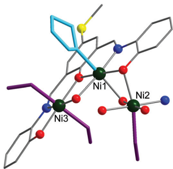
Fig. 3 A fragment of compound 1 representing pseudo-octahedral coordination geometries of the Ni(II) centres. For clarity, only one chelating Schiff-base ligand \text{L-SMe}^{3-} is explicitly depicted. The nickel, nitrogen, oxygen, and sulfur atoms are represented as ball-and-stick models. The terminal-coordinated solvent molecules are highlighted in different colours: MeOH, purple; THF, sky blue. Elemental colour code: C, grey; N, blue; O, red; S, yellow; Ni, dark green.
