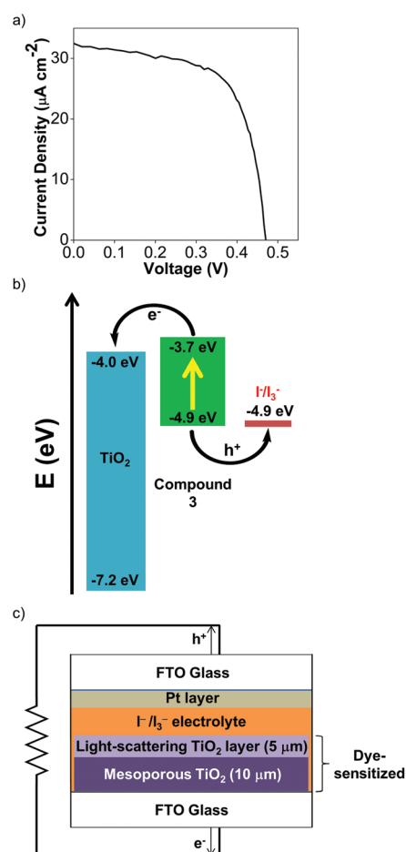
Fig. 7 (a) J - V plot for DSSCs after 3 has been adsorbed for dye-sensitization. (b) Band alignment for DSSC incorporated with 3 , showing the relative energy levels (in eV against vacuum) for 3 , \text{TiO}_2 , and the \text{I}^-/\text{I}_3^- electrolyte. (c) General device structure for the DSSCs prepared in this study.
