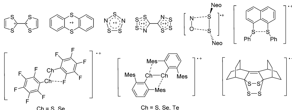
Fig. 88 Selected chalcogen radical cations, which were stabilized by WCAs.
