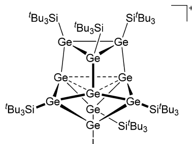
Fig. 50 Lewis structure of the 5-iodo-2,4,6,8,9,10-hexakis(tri-tert-butylsilyl)heptacyclo[4.4.0.0.1.3.0.2.5.0.3.9.0.4.7.0.8.10]decagerman-7-ylum ion.
