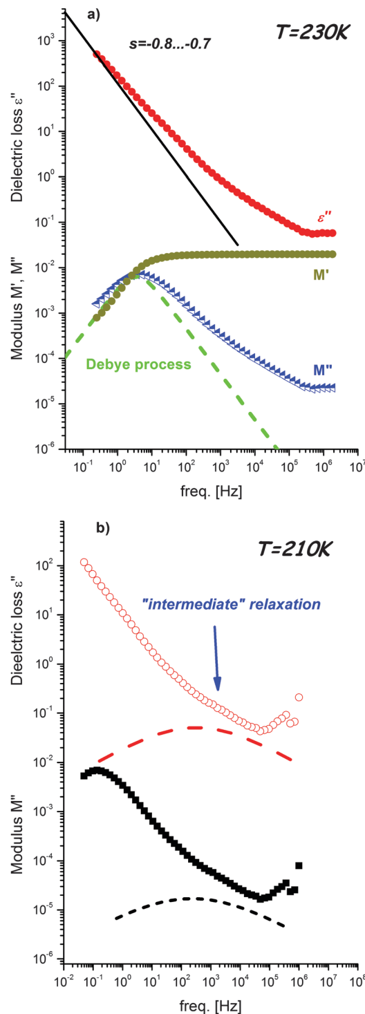
Fig. 3 (a) Comparison of the \varepsilon'' spectra with M' and M'' spectra measurements at 230 K. The straight line represents slope equal -1 ionic conductivity. Dashed curves represent the Debye process. (b) The \varepsilon'' and M'' spectra collected at 210 K. Dashed curves represent (as guide for the eyes) the “intermediate” relaxation process masked by the conductivity part.
