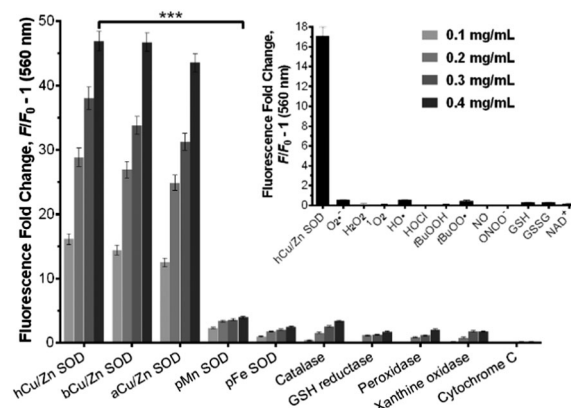
Fig. 2 Fluorogenic response of SODO upon binding to different proteins (at 0.1, 0.2, 0.3 and 0.4 mg mL -1 ) and metabolites (inset, ROS & RNS: 100 µM) in 20 mM Tris-HCl buffer (pH = 7.4). \lambda_{exc} : 460 nm, \lambda_{em} : 560 nm. Values are represented as means and error bars as standard deviations ( n = 3 ), *** for p < 0.001 .
