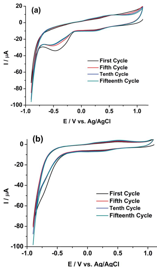
Fig. 8 Cyclic voltammograms of 5 mM \text{U(VI)} in 1 M \text{H}_2\text{SO}_4 on (a) rGO/GC and (b) GC electrodes at a scan rate of 50 \text{ mV s}^{-1} for (i) first, (ii) fifth, (iii) tenth and (iv) fifteenth cycle.
