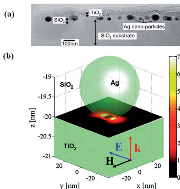
Fig. 4 (a) TEM cross sectional view showing TiO 2 film on Ag/SiO 2 core-shell on a SiO 2 substrate. (b) Simulation showing the near-field amplitude enhancement inside a TiO 2 substrate at the interface to a SiO 2 substrate where a Ag NP is embedded. The y-polarized illuminating plane wave propagates in the z-direction. Reprinted with permission from ref. 56.
