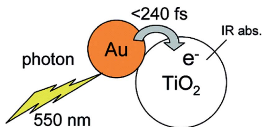
Fig. 3 Schematic representation of a gold nano dot attached on a TiO 2 nanoparticle, also indicating hot electron transfer process upon the excitation of LSPR. Figure reprinted with permission from ref. 59.
