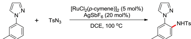
Scheme 164 Ru(III)-catalyzed C–H amidations of heteroaryl arenes.
