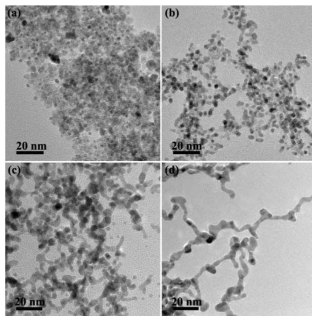
Fig. 7 TEM images of PtSn/SnO 2 CNs synthesized at 180\text{ }^{\circ}\text{C} for 0.5 h (a), 2 h (b), 4 h (c) and 24 h (d).
