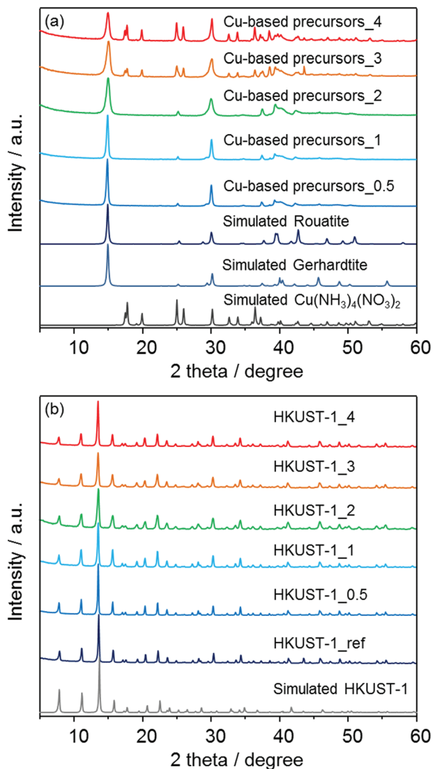
Fig. 3 XRD patterns of (a) the solvent insoluble Cu-based precursors (Cu-based precursors_X) with simulated patterns for \text{Cu}_2(\text{OH})_3\text{NO}_3 (rouatite and gerhardtite) and \text{Cu}(\text{NH}_3)_4(\text{NO}_3)_2 and (b) corresponding HKUST-1_X with HKUST-1_ref and simulated pattern for HKUST-1.
