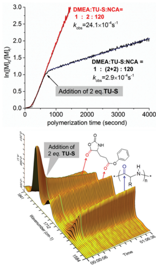
Fig. 6 \ln([M]_0/[M]_t) vs. time for the ROP of Glu-NCA initiated by DMEA/TU-S ( [M] = 0.19 M, [\text{Glu-NCA}]/[\text{TU-S}]/[\text{DMEA}] = 120/(2 + 2)/1 , 25^\circ\text{C} , \text{CH}_2\text{Cl}_2 ) and corresponding 3D kinetic behavior profile from in situ IR (the sampling interval of in situ IR is 10 seconds).
