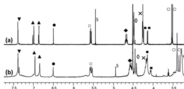
Fig. 1 1 H NMR spectra (500 MHz, 300 K) of (a) organosoluble Rim 3 ligand in CD 3 CN and (b) water-soluble WRim 3 ligand in D 2 O (2.6 mmol). (▼) HAr. “down”; (▲) HIm; (●) HAr. “up”; (○) NCH 3 ; (◊) CH 2 Im; (x) ArCH 2 O; (†) CH 2 N + Me 3 . S stands for solvent.
