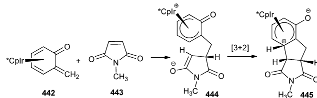
Scheme 97 Cycloaddition reaction of \text{Cp}^*\text{Ir}(\text{o-QM}) with N -methylmaleimide.
