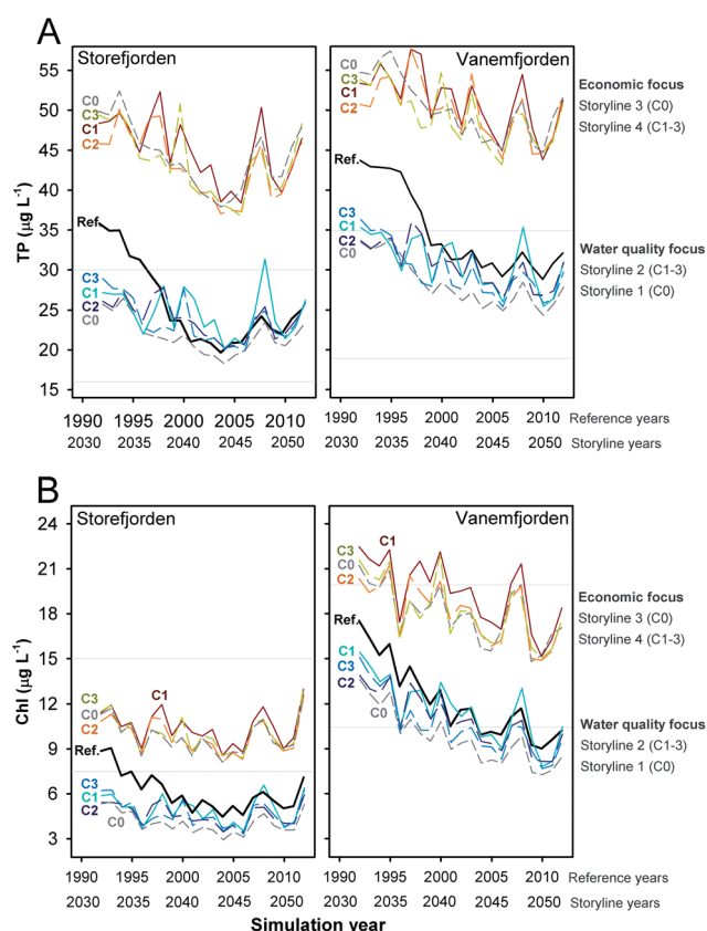
Fig. 7 Predicted yearly median total P (panel A) and chlorophyll (panel B) at Storefjorden (L1) and Vanemfjorden (L2) by the MyLake model without (C0; storylines 1 and 3) or with climate change predictions made using the HadRm3 (C1), the ECHAM5 (C2) or the BCM models (C3) as climate forcing (storylines 2 and 4) for the river-lake model network. The thick solid lines represent the reference conditions and the thin horizontal solid lines indicate the WFD thresholds specific to each basin (see Table 4).
