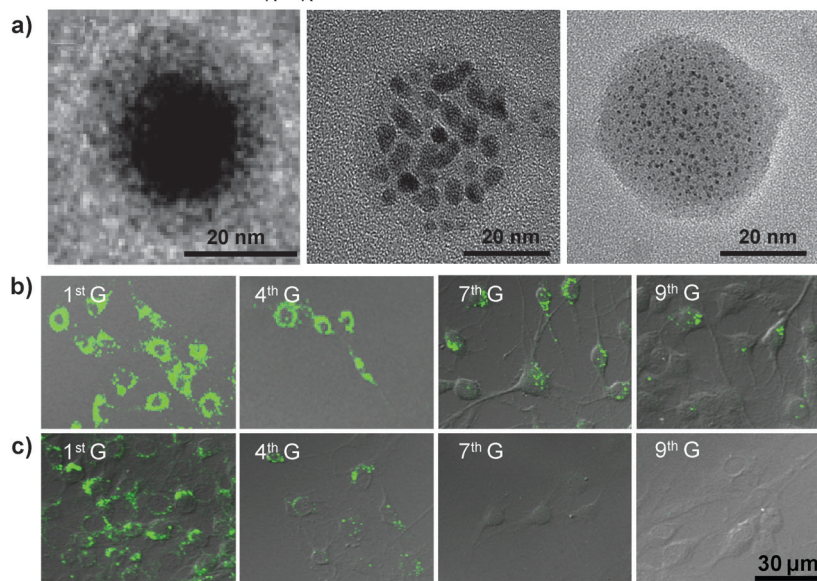
Fig. 7 Chemical structure of CP8 and (a) TEM images of the nanoparticles prepared from different concentrations of CP8 in the feed: 1.00, 0.50 and 0.25 mg mL -1 (from left to right) using DSPE-PEG as the matrix. Confocal images of MCF-7 cancer cells labeled with 2 nM (b) Tat- CP8 nanoparticles prepared using the DSPE-PEG-maleimide matrix or (c) Qtracker ® 585, after subculturing for different generations (G). All images in (b) and (c) share the same scale bar of 30 \mu m (reprinted with permission from ref. 95, Copyright 2013 Wiley-VCH).
