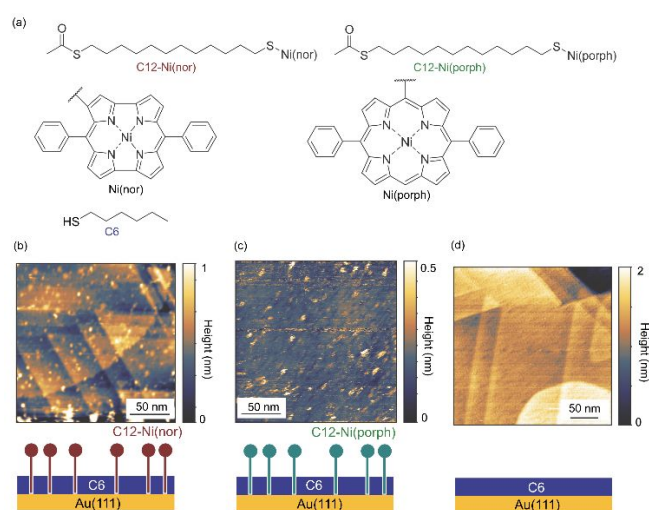
Fig. 1 (a) The chemical structures of hexanethiol (C6) and acetyl-protected dodecanethiol with the norcorrole Ni(II) moiety (C12-Ni(nor)) and with the porphyrin Ni(II) moiety (C12-Ni(porph)).
