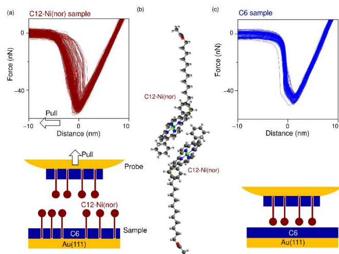
Fig. 2 (a,c) Force curves measured on C6 matrix with and without C12-Ni(nor). Adhesion force was defined as the maximum attraction (most negative force signal value) measured by the force curve. Schematics of the experimental systems are shown at the bottom. (b) Schematic illustration of the \pi -stack formation between C12-Ni(nor). Grey, white, blue, red, yellow, and green balls correspond to C, H, N, O, S and Ni atoms, respectively.
