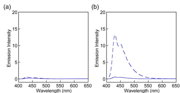
Fig. 4 PL spectra of the toluene solution of (a) Rot1 and (b) Rot3 before (dashed lines) and after (solid lines) heating for 3 h at 90 °C. The concentration of the solutions did not change upon heating. The PL spectra were recorded with the excitation light of 380 nm at r.t.
