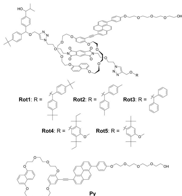
Fig. 2 Chemical structures of rotaxane-based supramolecular mechanophores Rot1-5 and ring reference Py .
