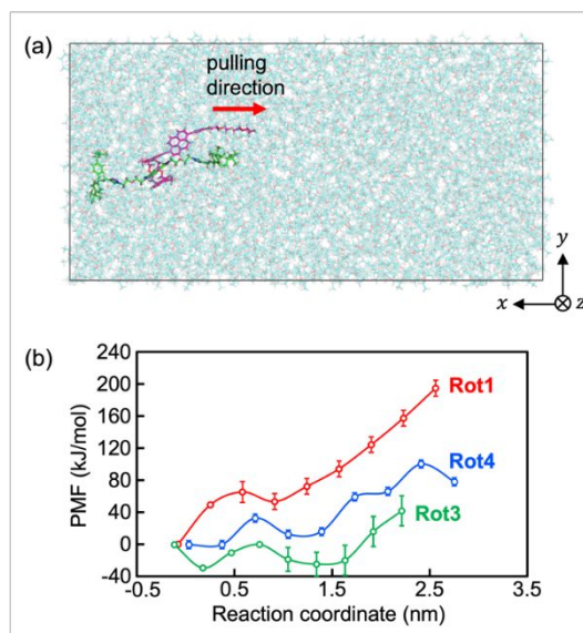
Fig. 6 (a) Steered MD simulation snapshot of Rot1 in the initial state. The ring and axle molecules are shown as purple and green sticks, respectively. Surrounding thin sticks in cyan represent DEE. (b) Potential of mean force (PMF) profiles of Rot1 , Rot3 , and Rot4 . The error bars depict only the statistical uncertainty from the connection of probability density by the weighted histogram method.
