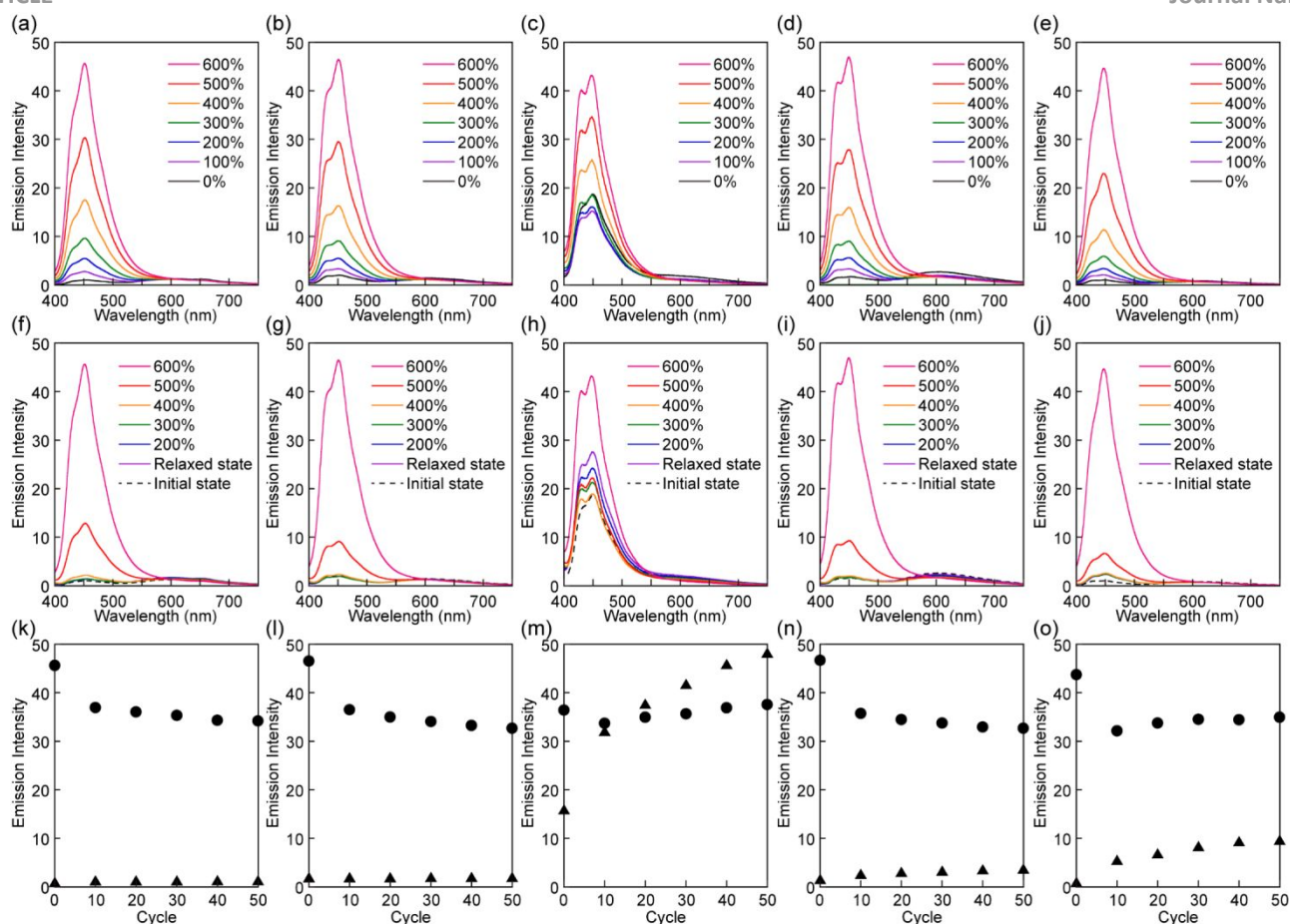
Fig. 5 Mechanoresponsive PL of films of Rot1-PU (a, f, k), Rot2-PU (b, g, l), Rot3-PU (c, h, m), Rot4-PU (d, i, n), and Rot5-PU (e, j, o). The top and middle panels show change in PL spectra upon the first stretching (top) and relaxation (middle) cycle. All spectra were recorded at the indicated strain. The bottom panels represent plots of the emission intensity at 450 nm recorded in cyclic tensile tests at strains of 600% (circles) and in the force-free state (triangles). All PL data were recorded with excitation at 380 nm.
