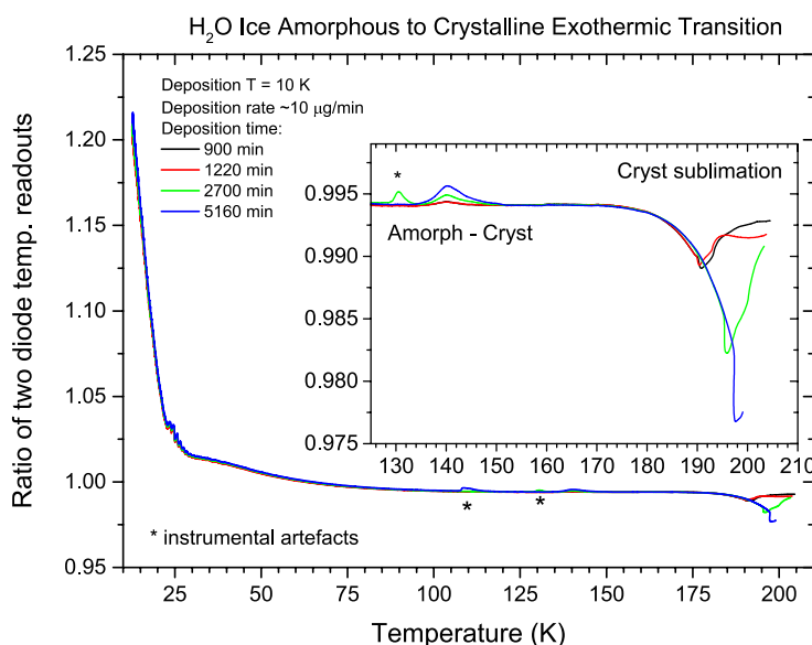
Figure 11: Differential calorimetry during 2K/min pure water ice annealing from amorphous to crystalline to sublimation transitions. Ratio of SD2/SD1 (SD= silicon diode for temperature readout) at various temperatures is plotted for four different ice experiments. SD2 is directly in contact with the ice, whereas SD1 acts as internal reference at the top of the sample holder. For an exothermic phase transition, this ratio is higher and for an endothermic phase transition it is smaller with respect to a common baseline ratio. We consistently see an exothermic transition between 130 and 150 K with maximum at 140 K due to the amorphous to crystalline phase transition. This peak position remains independent of ice thickness, but the transition intensifies with thickness as expected (more ice deposition mass induces a greater heat release and larger differences in the temperatures read at SD1 and SD2). We also observe the endothermic sublimation transition with an onset around 170 K, which also intensifies with thickness. The sublimation onset is the same in all cases, but the sublimation maximum shifts depending on thickness, since it is a surface-driven phenomenon and takes longer for thicker ices to complete the sublimation process. For thinner ice it maximizes at \sim 190 K, and moves to higher temperatures for thicker ice.
