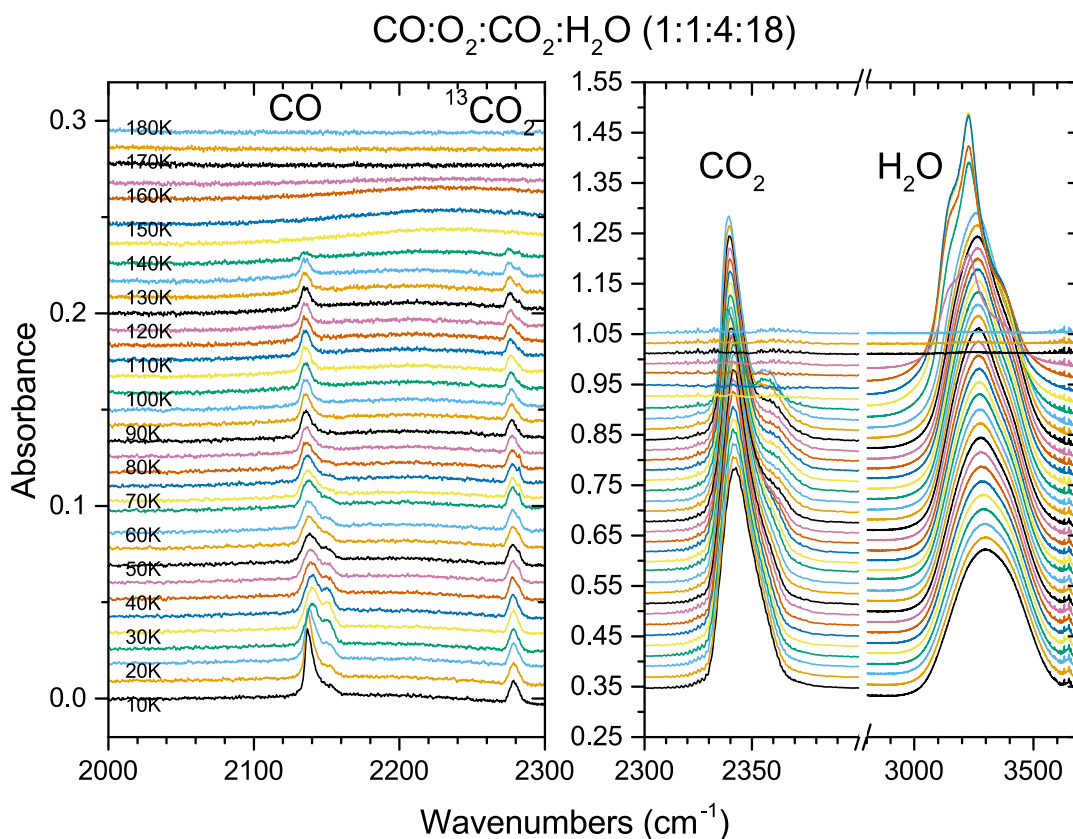
Figure 10: FTIR absorbance spectra of four component CO:O 2 :CO 2 :H 2 O mixed molecular ice during TPD. Spectra are stacked to provide clarity. CO absorption around 2140 cm -1 quickly splits into two components, the higher energy one disappearing by 90 K, indicating the lower energy part should be due to CO trapped in amorphous water-ice. CO 2 absorption at 2340 cm -1 starts as a single broad band and as the temperature increases a shoulder develops on the higher energy side, which becomes a clear band beyond CO 2 ice sublimation. Around 145 K all CO 2 sublimates and amorphous water ice band centered around 3250 cm -1 develops into a three-band structure, typical of crystalline water ice. Around 185 K, all the water ice sublimates, leaving no residue behind.
