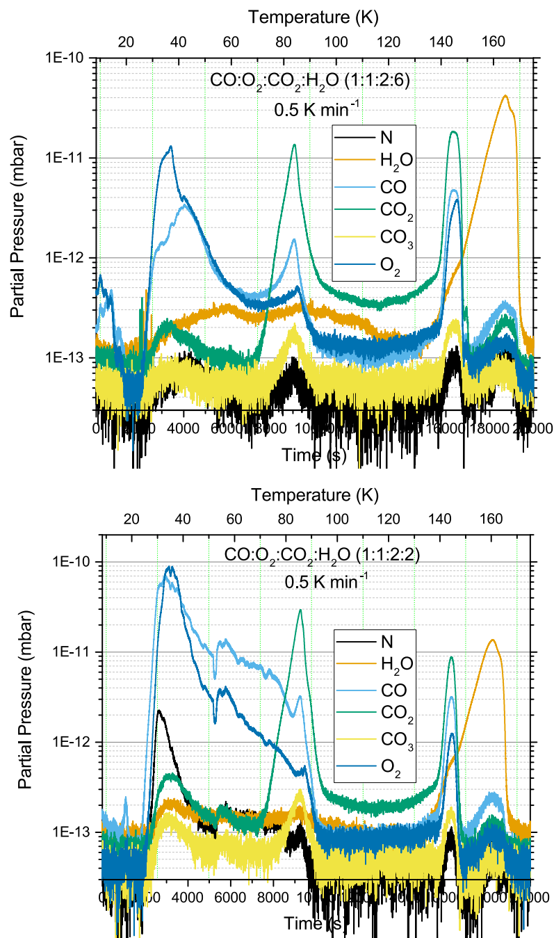
Figure 9: Mass spectral profiles during TPD from 10 K to 190 K of four component mixed molecular ices CO:O 2 :CO 2 :H 2 O.
