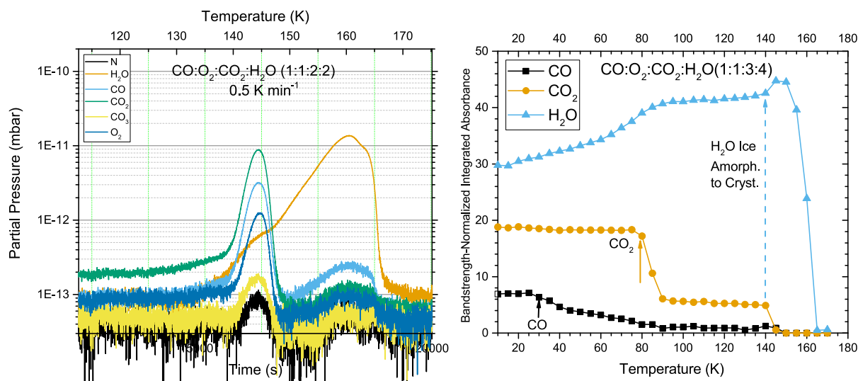
Figure 6: Zoomed-in part of the TPD-MS profiles (left) and integrated TPD-IR absorption intensities (right) of four-component CO:O 2 :CO 2 :H 2 O ice deposited at 10 K and heated at 0.5 K/min. In the left figure, we see between ~137 K and ~147 K a significant outgassing of trapped volatiles in amorphous water ice. In the right figure, we observe similar outgassing onset of CO (hence O 2 as well) at 30 K and gradual outgassing until CO 2 outgassing that occurs between 70 K and 90 K. Above 90 K, the amount of CO trapped in the amorphous ice is far less than CO 2 . The data confirm outgassing of almost all CO, O 2 , and CO 2 during crystallization of amorphous ice. During water-ice sublimation only a few percent of these volatiles are still trapped. This experiment demonstrates that if crystalline water ice in astrophysical environments were to be formed, it could accommodate a maximum of 5% of other volatiles in its lattice. If crystalline water ice is observed along with other ices, they must have been formed separately after amorphous water ice has been crystallized (i.e., subjected to temperatures above 120 K for a given amount of time, which is dependent on the maximum exposed temperature below 160 K under vacuum conditions). Please note that water ice integrated absorbance increases constantly and reaches its maximum around 150 K. This is less likely to be due to the increased band strength of water ice with temperature, but rather due to sublimation of a small amount of water from warmer parts of the cryostat and redeposition on the sapphire optical window. For the rest of the information on the figure details, please refer to Figure 3.
