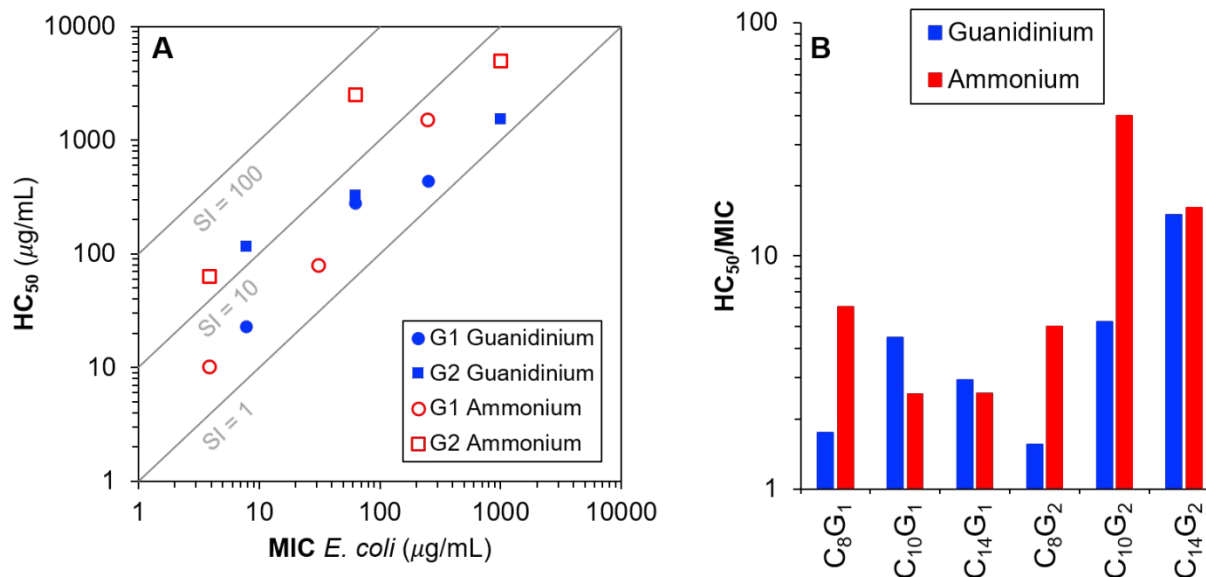
Figure 2. (A) Log-log Ashby plot of hemolytic activity against sheep red blood cells versus antimicrobial activity against E. coli and (B) bar chart of selectivity index, HC 50 /MIC, for the 1 st and 2 nd generation dendrons as a function of the chemical structure of their cationic charges.
