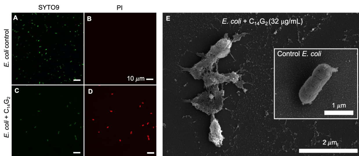
Figure 1. Confocal laser scanning microscopy images of (A, B) E. coli in PBS and (C, D) E. coli exposed to C_{14}G_2 at 32 \mu\text{g/mL} and (E) Scanning Electron Microscopy (SEM) images of E. coli exposed to C_{14}G_2 at 32 \mu\text{g/mL} compared to (inset) E. coli alone, both after fixation.
