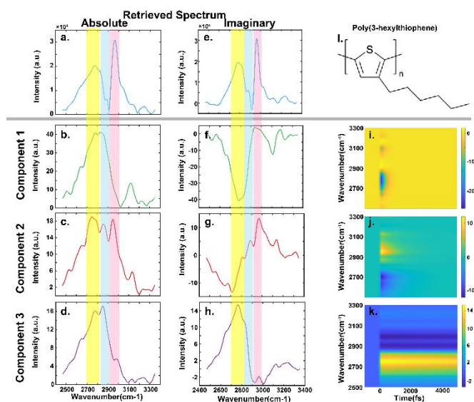
Figure 3. Retrieved spectral and dynamical components from an experimental transient VSGF scan on P3HT/Au interfaces. (a) The absolute static HD VSGF spectra of P3HT on Au had three major peaks, corresponding to electronic resonance (yellow), \text{CH}_2 FR (blue) and \text{CH}_3 AS (red). The transient spectral dynamics were decomposed into three components, including (i) coherent artifacts, (j) charge recombination and (k) charge separation. (b-d) The corresponding absolute spectral components showed the molecular peaks involved in each dynamic. A comparison between (e) the imaginary static VSGF spectra and (f-h) the imaginary parts of three transient spectral components shows the changes of spectral phase. (l) molecular structure of P3HT
