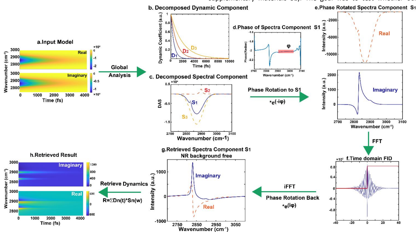
Figure 1. Flow chart of the data analysis method. The (a) initial input data was decomposed by global analysis (Glutaran) into various (b) dynamics and (c) spectral components. By inspecting the spectral components, S_1 contained a broad background which is the NR signal, and a small dip corresponding to a molecular feature, S_2 only had a sharp molecular feature and S_3 was only NR signal. Thus, we only needed to process S_1 to separate the molecular features from NR signals. We then determined the phase \phi of NR signal from (d) the phase plot of S_1 . The flat phase region represented the NR phase, which should be a constant. By applying a phase rotation, (e) the NR signal was fully rotated to the real part of the phase rotated S_1 , whereas the imaginary part was composed of a molecular resonance. Then, we Fourier transformed only the imaginary spectra to get (f) the time domain free induction decay (FID) and applied a Heaviside function (red in f) to impose causality. The FID after causality was inverse Fourier transformed back and applied an inverse phase rotation to restore the original spectral phase. (g) The retrieved S_1 now was free of NR signal and only composed of molecular responses. The retrieved molecular dynamics, free from NR dynamics, could be composed of three spectral and dynamical components by equation: R = \sum D_n(t) \otimes S_n(\omega) , where \otimes is the outer products of vectors and D_n and S_n are the dynamical and spectral components n , after NR removal.
