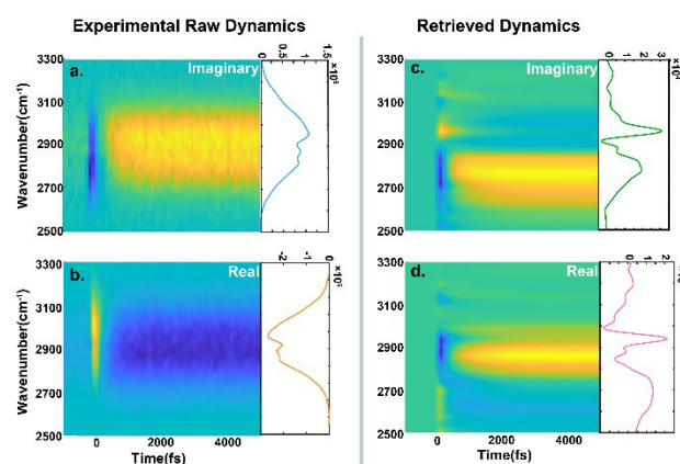
Figure 4. A comparison between imaginary and real parts of (a and b) experimental raw dynamics of charge transfer at P3HT/Au interfaces (and corresponding linear VSFG spectra, right) and (c and d) retrieved molecular dynamics (and corresponding molecular contribution to the linear VSFG spectra, right). The retrieved results (c and d) show the dynamics of three molecular resonance of P3HT, which is overwhelmed by the dynamics of large NR background in a and b.
