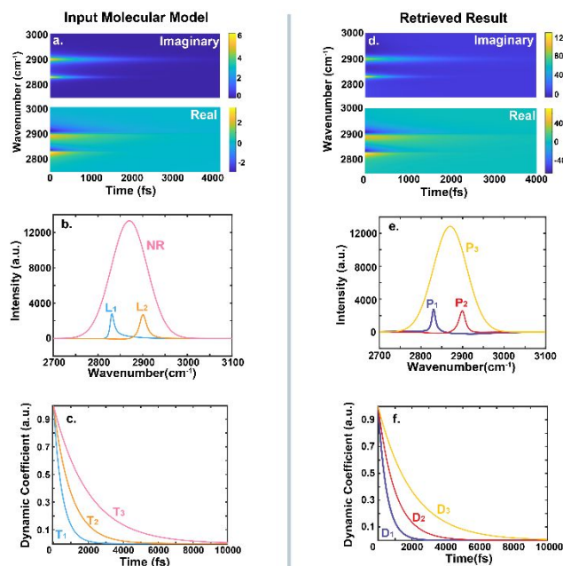
Figure 2. Comparison of (a-c) model input and (d-f) retrieved results. The full dynamics of model input is plotted in Fig.1.a, which was composed according to equation 2, by three spectral components and three dynamic components. After retrieval described in Fig.1, the retrieved (e) spectral and (f) dynamic components matched well with the initial input (b) and (c). Finally, based on the relationships between P and D, we could (d) reconstruct molecular dynamics, which extracted (a) the molecular dynamics of model input from the overall dynamics of the model (Fig.1a) well.
