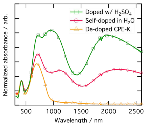
Figure 4. UV-vis-NIR absorption spectra of CPE-K films at various levels of doping, normalized using the peak at 410 nm.
