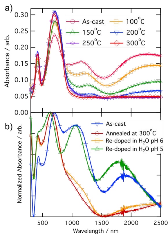
Figure 5. UV-vis-nIR absorption spectra of CPE-K with a) annealing for 30 minutes and b) after re-doping the film under oxygen-free conditions, normalized to peak at \sim 690 nm
