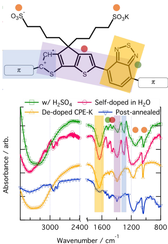
Figure 3. ATR-IR spectrum and corresponding functional group vibrations denoted by color on the chemical structure on the right.
