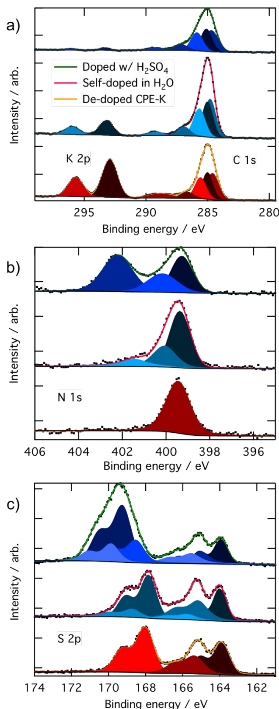
Figure 2. High resolution XPS spectra of a) C 1s and K 2p 3/2 , b) N 1s, and c) S 2p 3/2 and their Voigt fitting profiles of CPE-K w/ H_2SO_4 added, self-doped CPE-K, and de-doped CPE-K on ITO with a film thickness of 20 nm. Black dots are experimental data and the colored lines are overall fits obtained with a peak-fitting routine.
