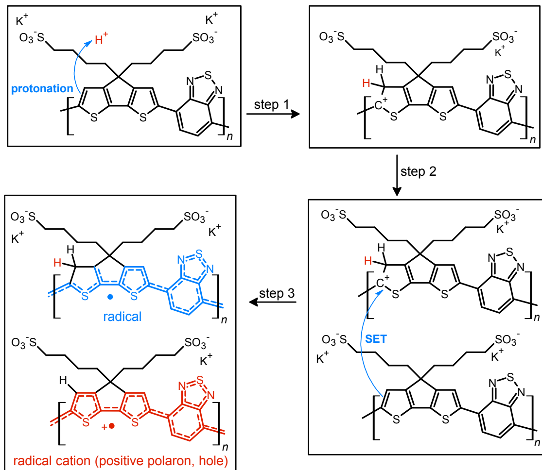
Figure 1. Proposed schematic representation for protonic acid doping of CPE-K, including hypothesized transient intermediates that follow step 1 and step 2. The system can then undergo single electron transfer (SET) to arrive at the final species.
