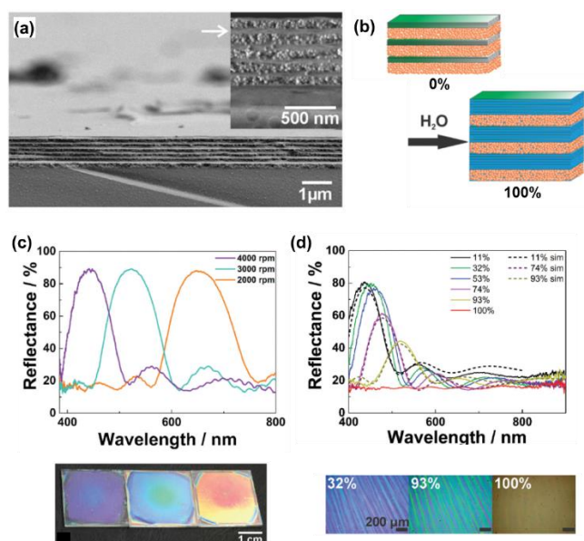
Fig. 5. Soft layered materials with flexibility in vertical direction for sensing applications based on the structural color. 73 (a) Cross-sectional scanning electron microscopy images of the layered architectures consisting of the exfoliated phosphatoantimonic-acid nanosheets and silica particles fabricated by spin coating at 4000 rpm. (b) Schematic illustration of the humidity sensing mechanism. (c) Optical spectra and photographs of the stackings fabricated by spin-coating at 2000, 3000, and 4000 rpm (from left to right in the photographs), respectively. (d) Experimental (solid spectra) and simulated (dashed spectra) reflectance spectra of the stacking at different humidity. (e) Microscope images at humidity 32%, 93%, and 100%, respectively. Reprinted with permission from Wiley-VCH. 73
