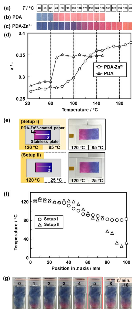
Fig. 15 Real-time 2D and 3D temperature-distribution imaging by the PDA-Zn 2+ -coated devices. (a) Sample temperature. (b,c) Photographs of the PDA- and the PDA-Zn 2+ -coated filter paper with changes of temperature. (d) Relationship between the temperature and x value of the PDA (triangles) and PDA-Zn 2+ (circles) estimated from the image analysis. (e) Experimental setup and photographs of the two different temperature distributions on the 2D surface, namely the setups (i) and (ii). (f) Relationship between the position in z axis and temperature in the setups (i) (circles) and (ii) (triangles). The x values of the PDA-Zn 2+ -coated filter paper were converted to temperature by using the relationship in Fig. 15d. (g) Time-course color change of the PDA-Zn 2+ -coated cotton in a glass bottle after the setting on the temperature-controlled stage at 150 °C. Reprinted with permission from ref. 78. Copyright 2020 American Chemical Society.
