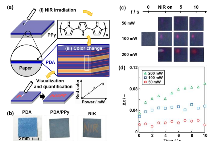
Fig. 17 Visualization and quantification of NIR using PPY/PDA-coated paper. (a) Structure of the device consisting of layered PDA with PPY coating and its NIR visualization mechanisms with the irradiation (i), photothermal generation (ii), and color change (iii). (b) Photographs of the PDA-coated paper (left), after the PPY coating for 15 min (center), and after writing the characters with irradiation using a NIR laser pointer (808 nm) (right). (c) Photographs before ( t = 0 ) and after the irradiation (NIR on t < 0.5 s and t = 5, 10 s) of NIR (50, 100, 200 mW). (d) Time-dependent changes of the \Delta x value with irradiation of 50 (red circle), 100 (blue square), 200 mW (green triangle) NIR. Reprinted from ref. 84 published by The Royal Society of Chemistry.
