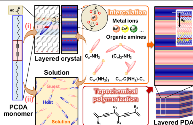
Fig. 7. Schematic illustration of the intercalation route (i) and self-organization route (ii) for preparation of the layered composites based on PDA with topochemical polymerization. Reprinted with permission from Wiley-VCH and Elsevier. 79,82,85
