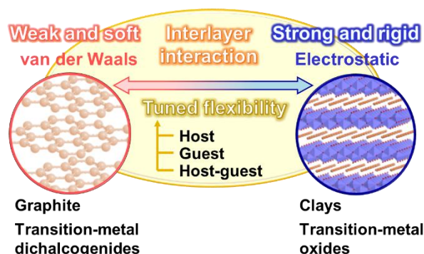
Fig. 2. Flexibility of the layered structures based on the interlayer interactions. Typical layered compounds are classified into the soft and rigid types originating from van der Waals and electrostatic interactions between the layers, respectively.
