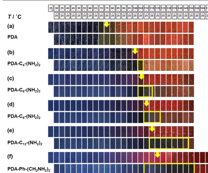
Fig. 11. Photographs of the alkyl-diamine-intercalated PDA samples with changes of the temperature by the protocol including heating (the upper panels) and subsequent cooling (the lower panels) as shown in the top part. The yellow arrows indicate the color-change temperature to red recognized by the naked eye. The yellow frames in the lower panels show the reversible color change to the original blue. Reprinted with permission from Springer Nature. 83
