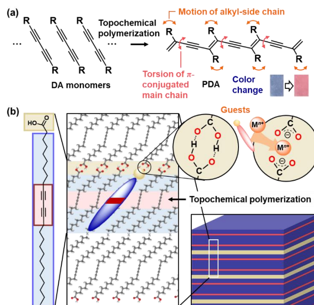
Fig. 6. Schematic illustration of the layered PDA. (a) DA monomer, its topochemical polymerization, and molecular motions with the application of external stimuli. (b) Layered crystal structure of PCDA, an amphiphilic DA monomer, intercalation of cations in the interlayer space consisting of the carboxy groups, and topochemical polymerization.
