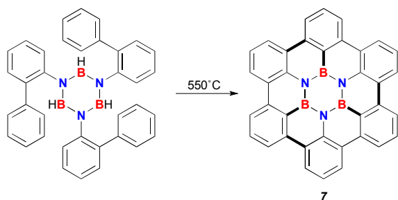
Scheme 5. BN-hexa-peri-hexabenzocoronene.
