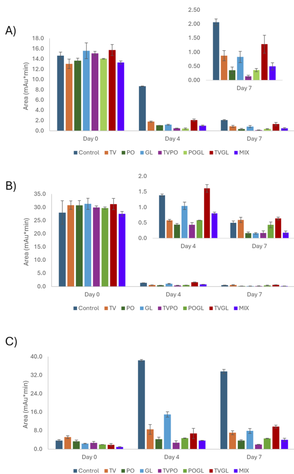
Fig. 1 Degradation of: (A) PAP; (B) PAOC; (C) coupling product.
