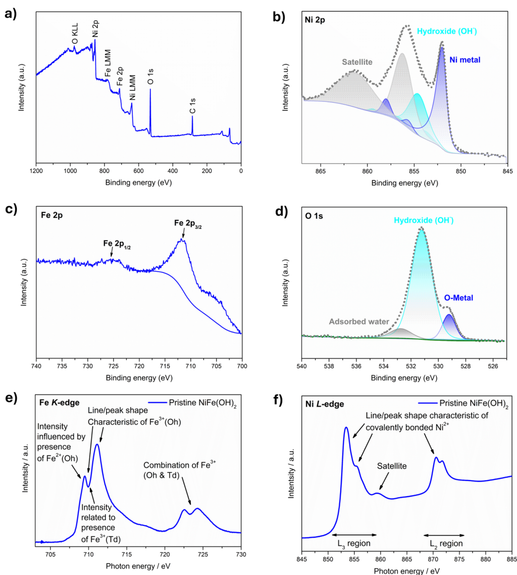
Fig. 3 (a) Survey scan of the XPS spectrum of \text{NiFe(OH)}_2 obtained on a carbon plate. And fitting results of the high-resolution scans in the (b) Ni 2p region (c) Fe 2p region (d) O 1s region (e) normalised Fe K-edge XANES spectra for \text{NiFe(OH)}_2 (f) normalised Ni L-edge XANES spectra for \text{NiFe(OH)}_2 .
