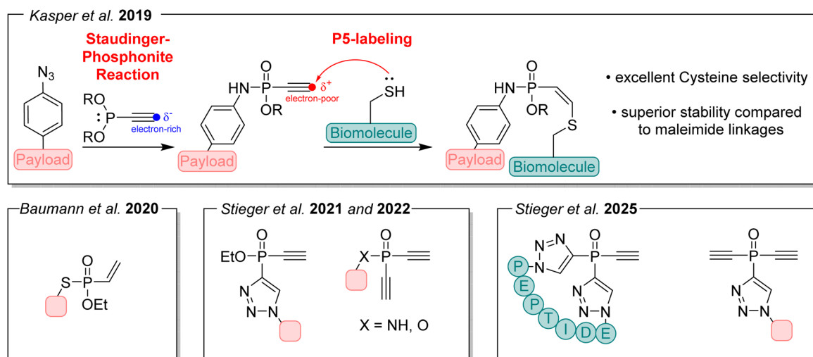
Fig. 2 Synthesis of a P5-electrophile (ethynyl-phosphonamidate) followed by cysteine-selective conjugation. Various P5 reagents developed subsequently are shown underneath. 8,14–17
