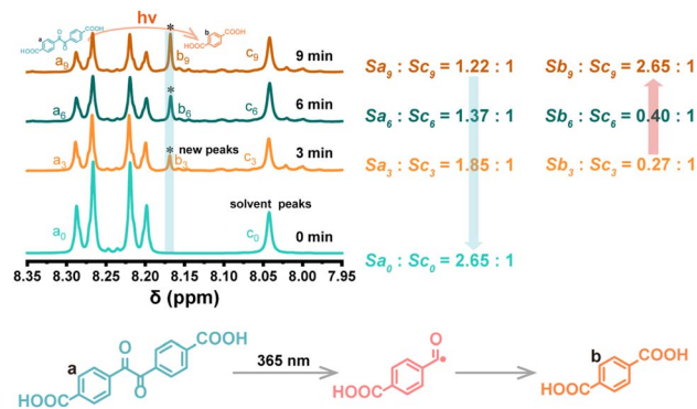
Fig. 2 Characterization of products after BS irradiation. ^1\text{H} NMR (400 MHz) spectra of BS in DMF- d_6 after different irradiation times using an external UV torch light ( 317.5 \text{ mW cm}^{-2} ).
