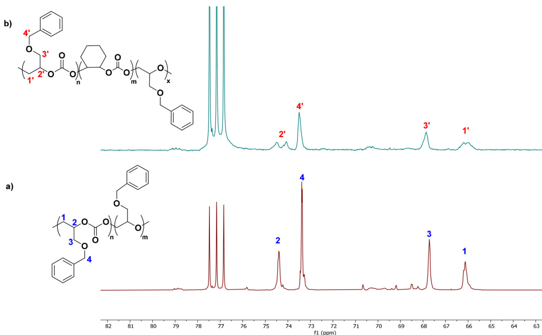
Fig. 5 Representative ^{13}\text{C}\{^1\text{H}\} NMR spectra (100 MHz, \text{CDCl}_3 , 23 °C) of a P(BnGEC) copolymer (a-bottom, Table 2, entry 7) and a P(BnGEC-co-CHC) terpolymer (b-top, Table 3, entry 3) synthesized with \text{BEt}_3/\text{PPNCl} catalyst system, showing the notable splitting of the backbone methylene ( \text{C1}/\text{C1}' ) and methine ( \text{C2}/\text{C2}' ) resonances in the terpolymer in comparison to its copolymer analogue.
