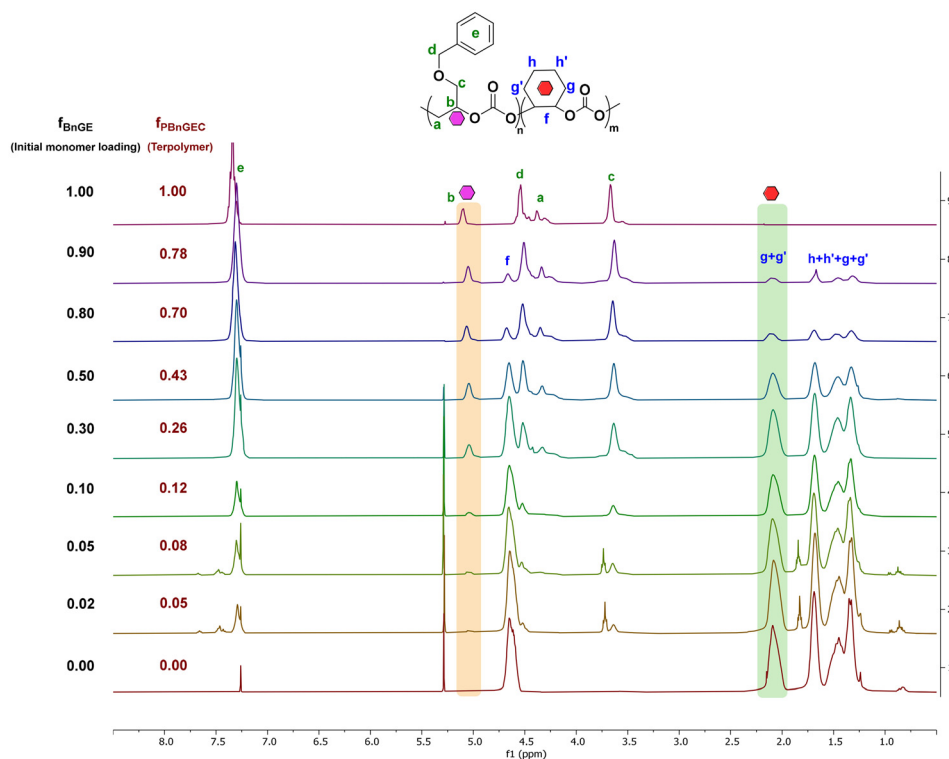
Fig. 4 ^1\text{H} NMR spectra (400 MHz, \text{CDCl}_3 , 23 °C) of P(BnGEC-co-CHC) terpolymers synthesized with the \text{BEt}_3/\text{PPNCl} system at various BnGE/CHO loadings (Table 3).
